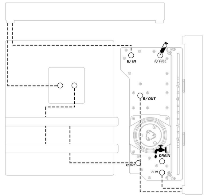
X-FLOW CONFIGURATION 1
