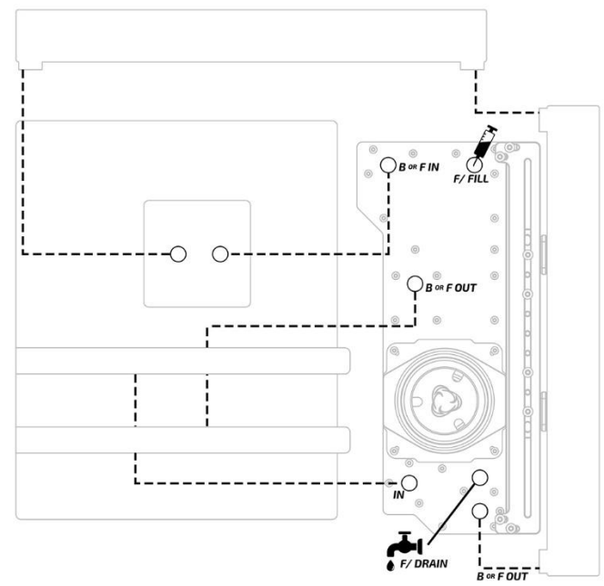
X-FLOW CONFIGURATION 1
