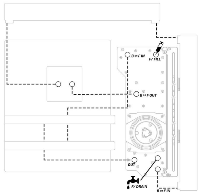
X-FLOW CONFIGURATION 2
