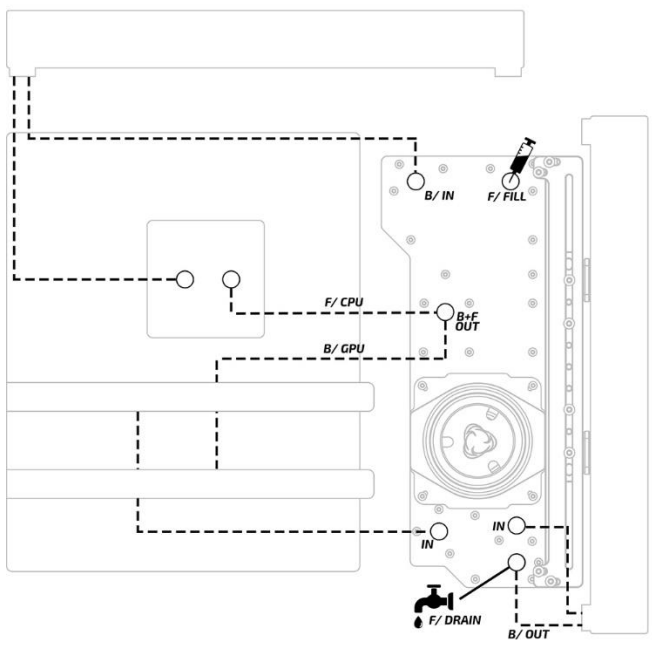
PARALLEL CONFIGURATION 1
