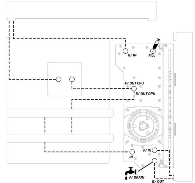
BOTH SIDES DUAL D5 PARALLEL CONFIGURATION
