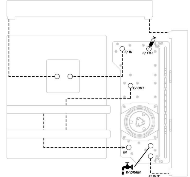
BOTH SIDES DUAL D5 PARALLEL CONFIGURATION
