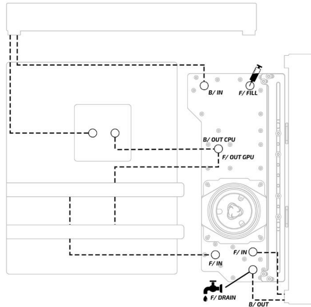
DUAL LOOP STANDARD CONFIGURATION
