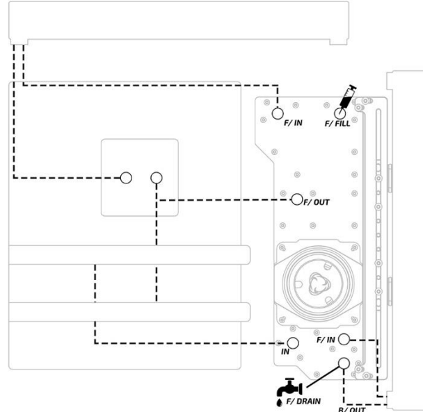
DUAL LOOP STANDARD CONFIGURATION
