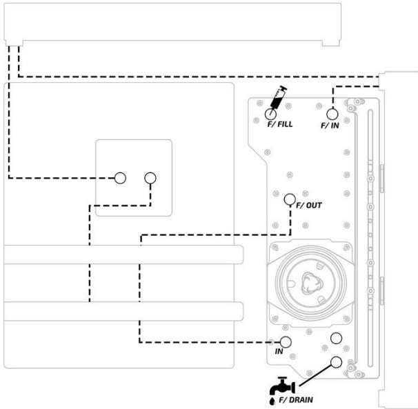
SINGLE LOOP X-FLOW CONFIGURATION 2
