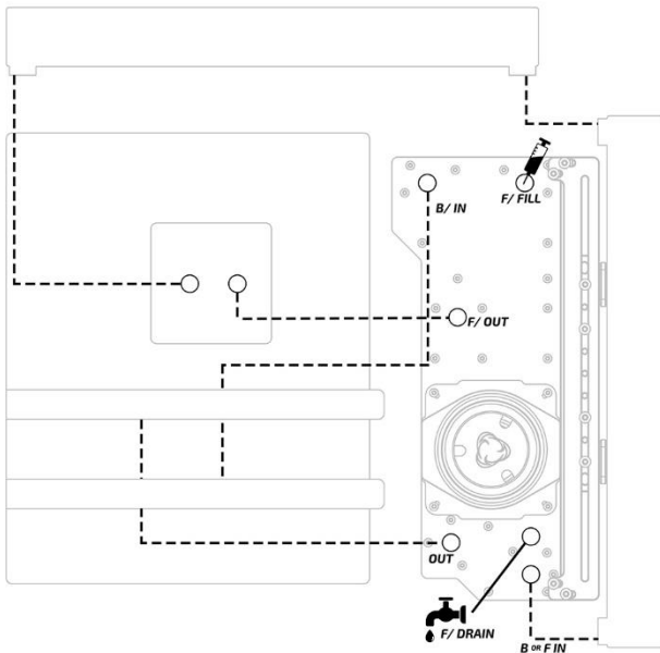
SINGLE LOOP X-FLOW CONFIGURATION 2
